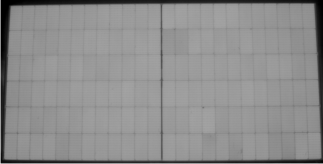
Fig. 7 EL photo of module No.1 Serial number: ASA22190402036
