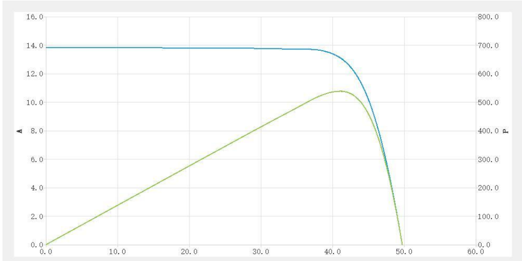
Fig. 5 IV curve of module No.1 Serial number: ASA22190402036
