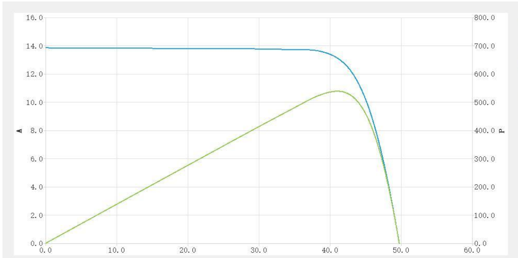
Fig. 6 IV curve of module No.2 Serial number: ASA22190402037
