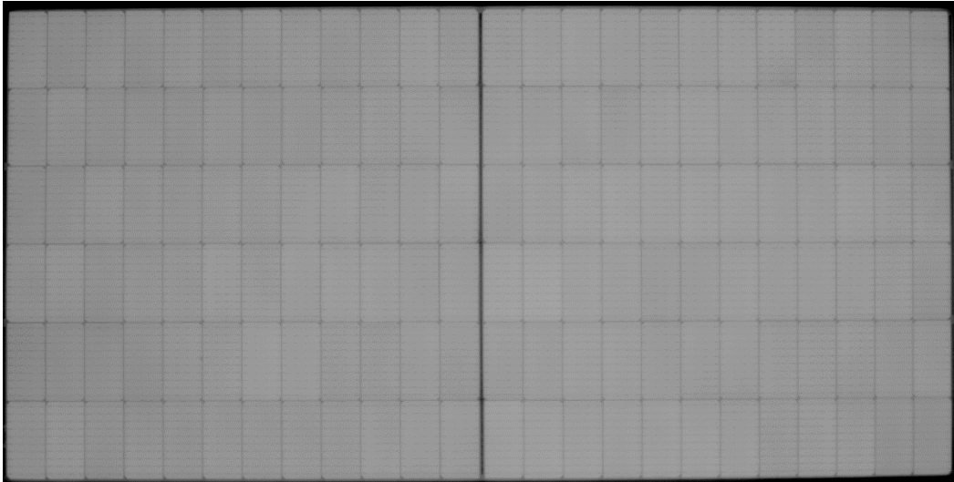
Fig. 8 EL photo of module No.2 Serial number: ASA22190402037
